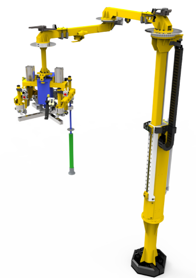
Transfer and Assembly of Foundry Molds
