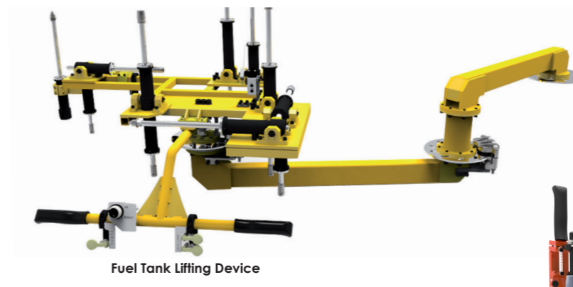
Fuel Tank Lifting Device
